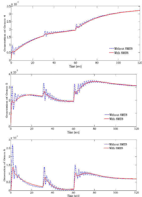
Fig.9: Generation of Gencos of Area II during contract violation
