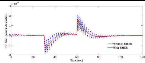
Fig.7: Comparison of Frequency deviations and tie line power error deviations during contract violation
