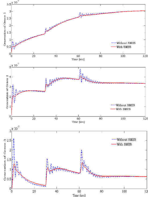
Fig.8: Generation of Gencos of Area I during contract violation
